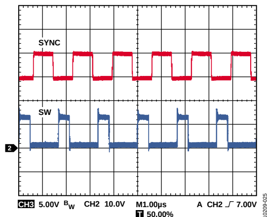
Figure 25. External Synchronization
