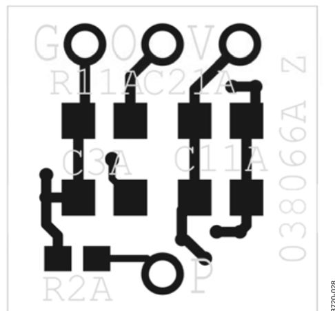
Figure 16. ADPD2211 Evaluation Board Bottom Layer
