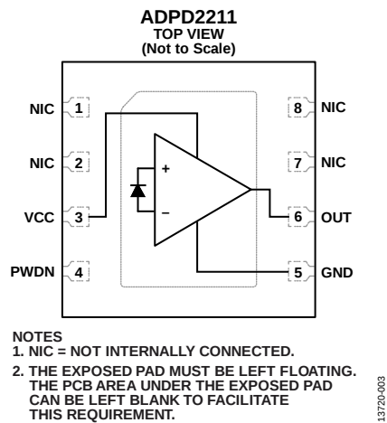
Figure 3. Pin Configuration
