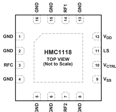
Figure 5. Pin Configuration
