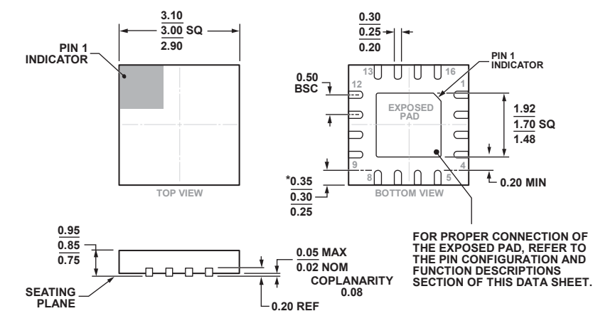
Figure 20. 16-Lead Lead Frame Chip Scale Package [LFCSP_WQ] 3 mm x 3 mm Body, Very Very Thin Quad (CP-16-38)
