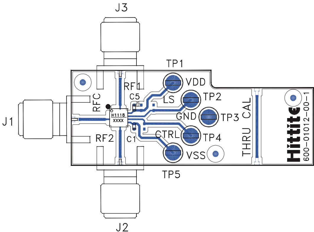
Figure 19. EV1HMC1118LP3D Evaluation PCB
