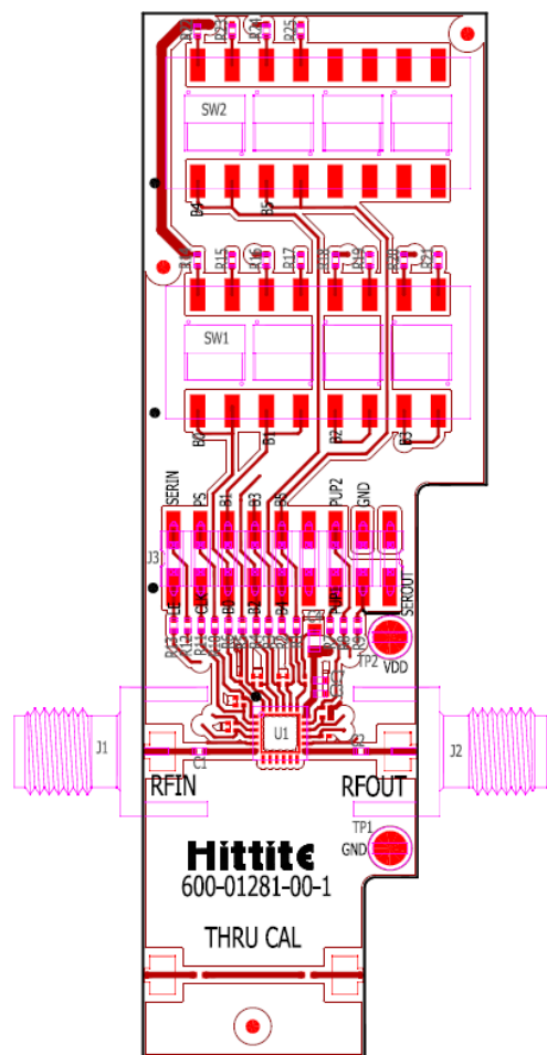
Figure 29. Evaluation Board Layout—Top View
