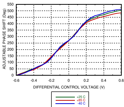
Phase Shift vs. Temperature [1][2][3][4]
