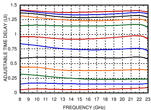
Time Delay vs. Control Voltage @ V_{DCP}=2.7V to 3.9V with 0.1V step [1][2]
