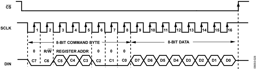
Figure 15. Writing to an 8-Bit Register
