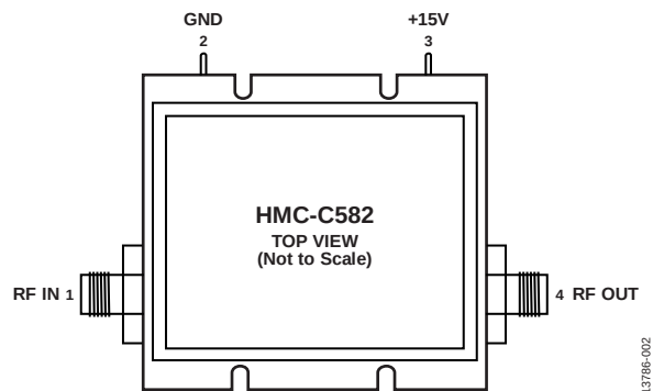
Figure 2. Pin Configuration
