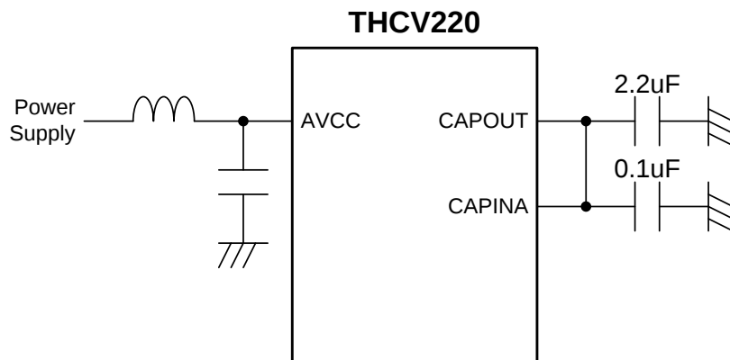
Figure 1. Connection of CAPOUT, CAPINA and Decoupling Capacitor
