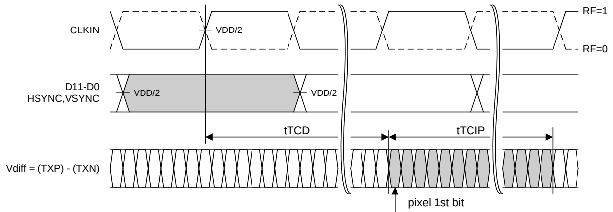
Figure 21. THCV231-Q Latency
