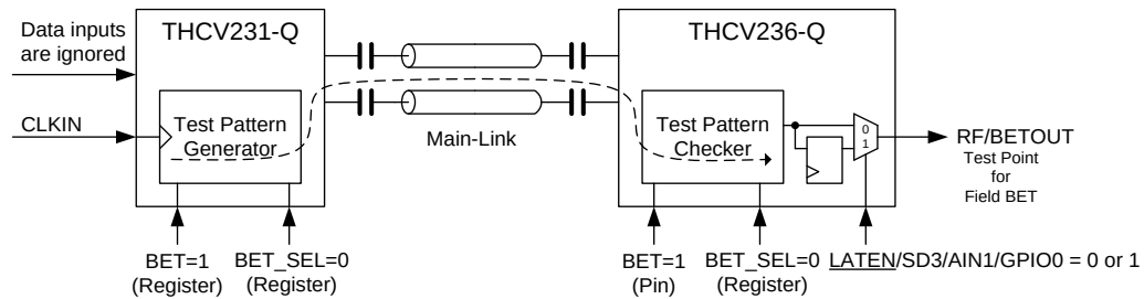
Figure 3. Main-Link Field BET Configuration
