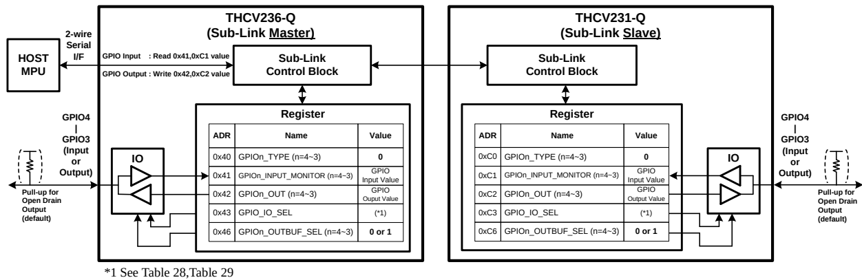
Figure 12. Programmable GPIO
