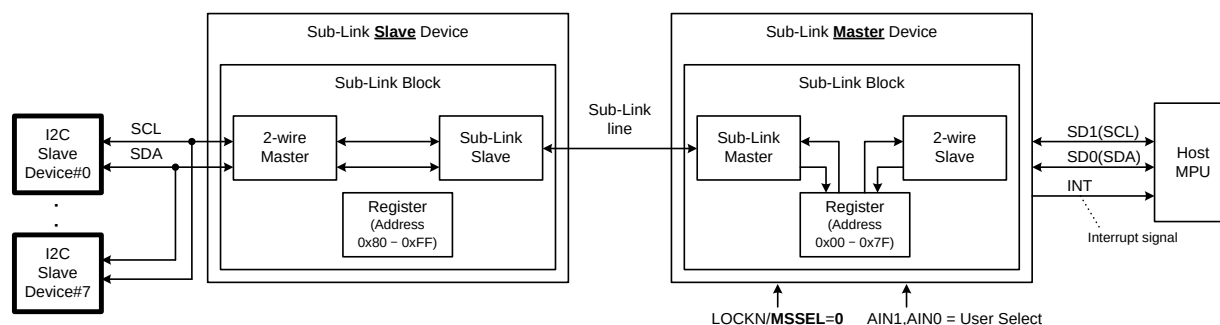
Figure 10. Host to 2-wire serial Slave devices connected to Sub-Link Slave device access configuration
