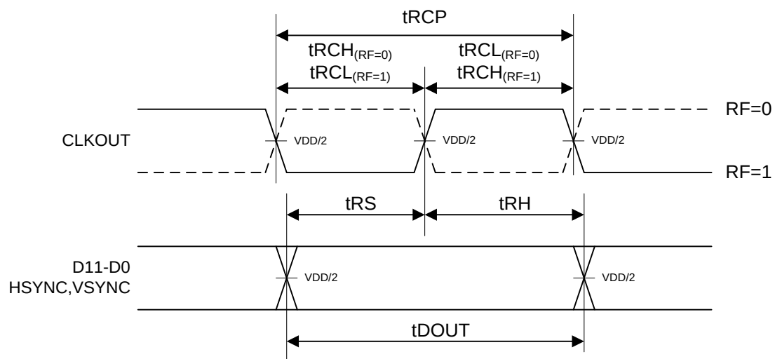
Figure 16. LVC MOS Output Switching Timing Diagrams
