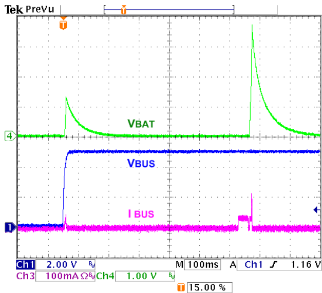
Figure 17. No Battery at V_{BUS} Power-up; FAN5400, FAN5403
