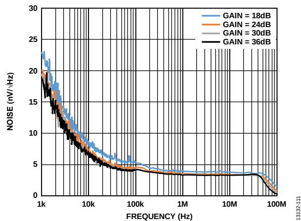
Figure 10. Input Referred Noise vs. Frequency
