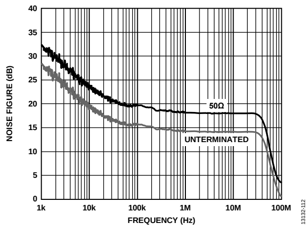
Figure 11. Noise Figure vs. Frequency
