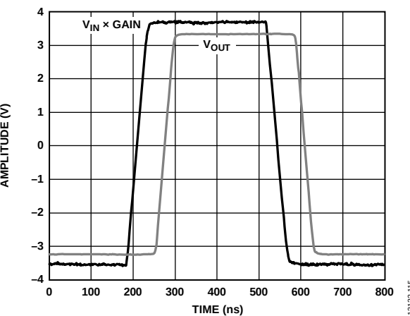
Figure 14. Overdrive Recovery
