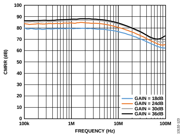
Figure 22. CMRR vs. Frequency at Various Gains
