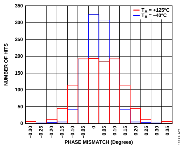
Figure 6. Distribution of Channel to Channel Phase Matching
