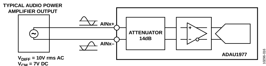
Figure 17. Connecting the Line Level Inputs—Differential DC-Coupled Case
