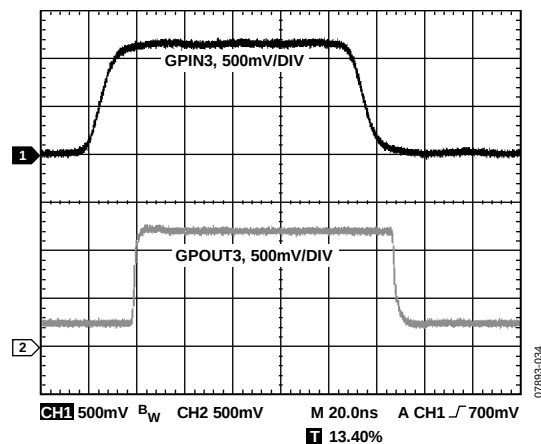
Figure 34. GPOUT3 Output vs. GPIN3 Input, V_{IN2} = 1.8\text{ V} , V_{IN3} = 1.2\text{ V} , 600\text{ }\Omega Pull-Up, CH1 = GPIN3, CH2 = GPOUT3
