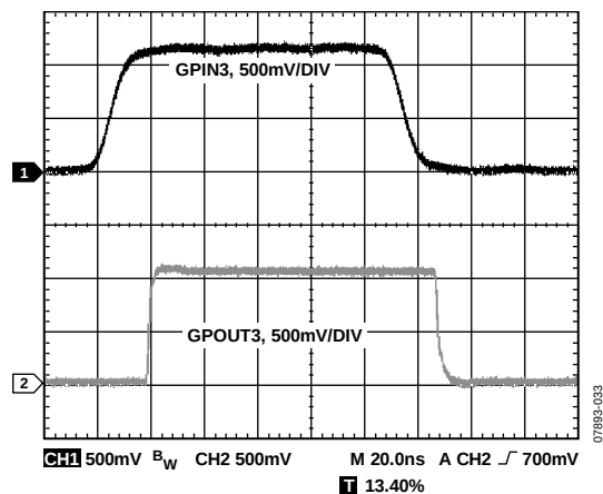
Figure 33. GPOUT3 Output vs. GPIN3 Input, V_{IN2} = 1.8\text{ V} , V_{IN3} = 1.2\text{ V} , 600\text{ }\Omega Pull-Down, CH1 = GPIN3, CH2 = GPOUT3
