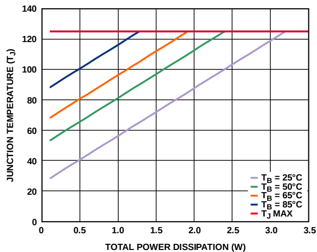
Figure 77. SOIC
