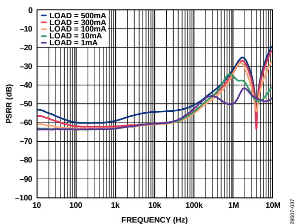
Figure 42. Power Supply Rejection Ratio vs. Frequency, V_{OUT} = 5\text{ V} , V_{IN} = 6\text{ V} Adjustable
