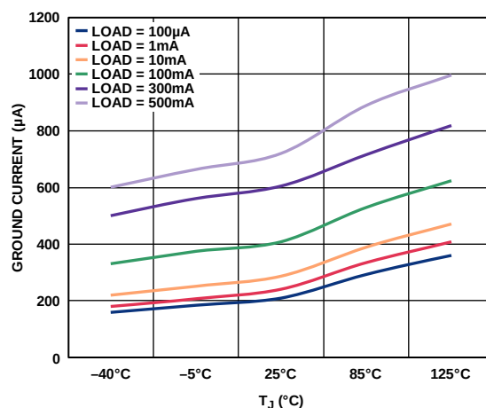
Figure 8. Ground Current vs. Junction Temperature
