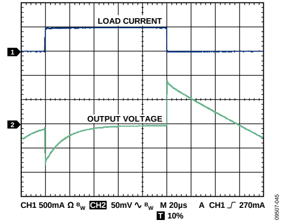
Figure 50. Load Transient Response, C_{IN} , C_{OUT} = 1\text{ }\mu\text{F} , I_{LOAD} = 1\text{ mA to } 500\text{ mA} , V_{OUT} = 1.8\text{ V} , V_{IN} = 5\text{ V}
