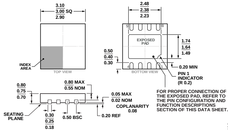
Figure 80. 8-Lead Lead Frame Chip Scale Package [LFCSP_WD] 3 mm × 3 mm Body, Very Very Thin, Dual Lead (CP-8-5)
