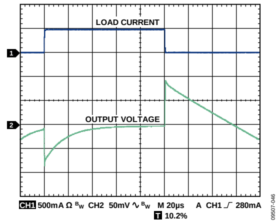
Figure 51. Load Transient Response, C_{IN} , C_{OUT} = 1\text{ }\mu\text{F} , I_{LOAD} = 1\text{ mA to } 500\text{ mA} , V_{OUT} = 3.3\text{ V} , V_{IN} = 5\text{ V}
