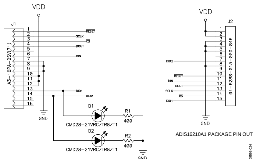
Figure 25. Electrical Schematic
