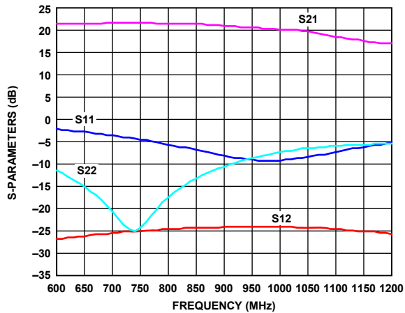
Figure 27. Typical S-Parameters, Log Magnitude
