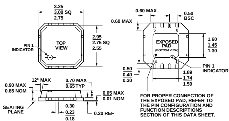
Figure 65. 8-Lead Lead Frame Chip Scale Package [LFCSP_VD] 3 mm x 3 mm Body, Very Thin, Dual Lead (CP-8-2) Dimensions shown in millimeters
