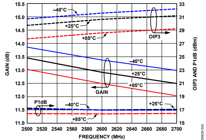
Figure 43. Gain, OIP3, and P1dB vs. Temperature
