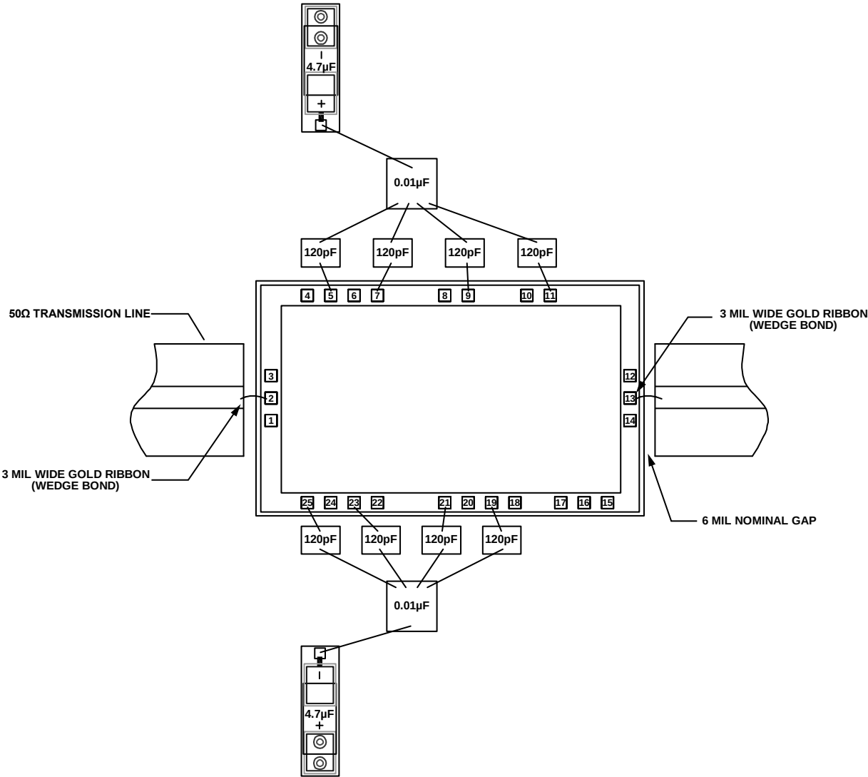
Figure 41. Assembly Diagram
