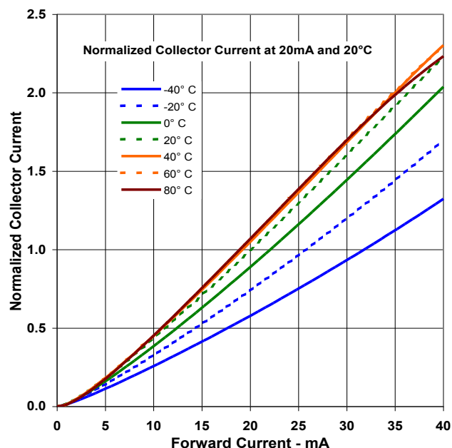
OPB701 - Normalized Collector Current vs Forward Current vs Temperature
