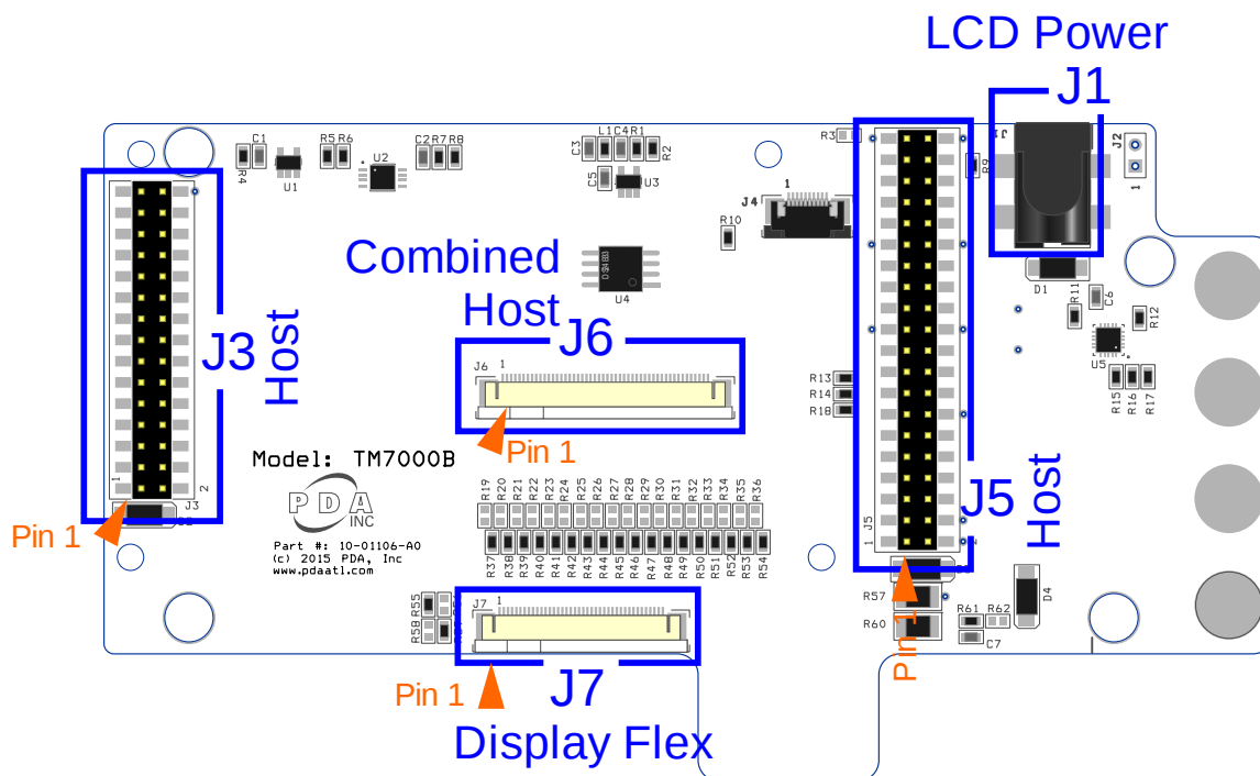
Figure 1 - PCB Connectors
