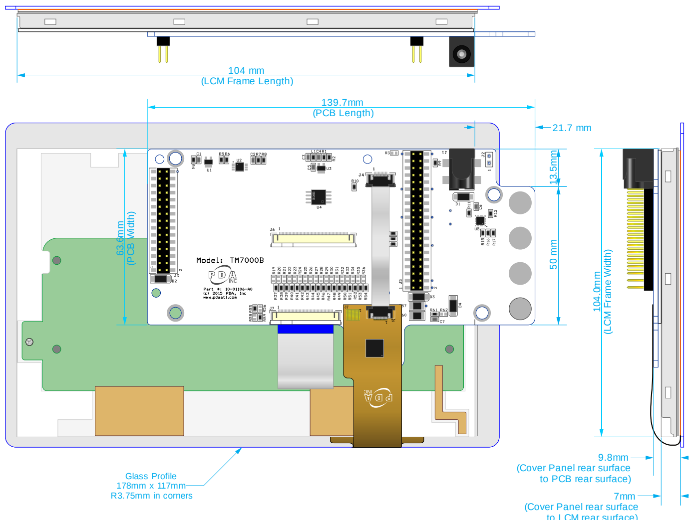
Figure 6 – Module Dimensions
