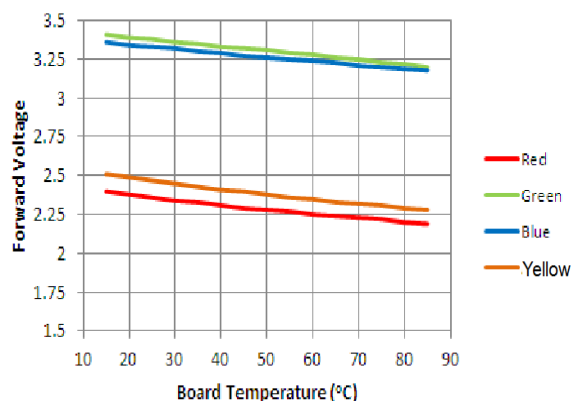
Forward Voltage vs. Thermal Pad Temperature @350mA
