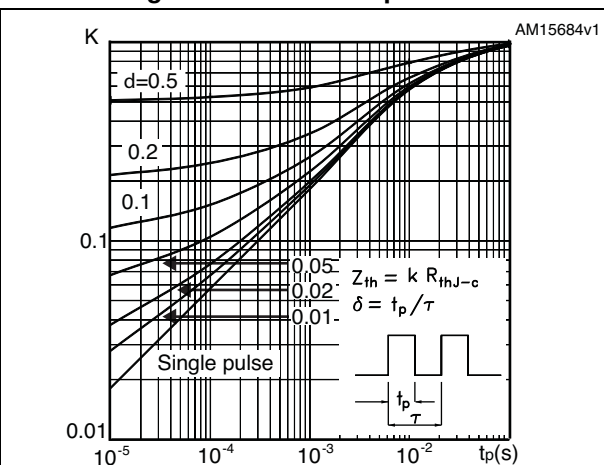
Figure 3. Thermal impedance
