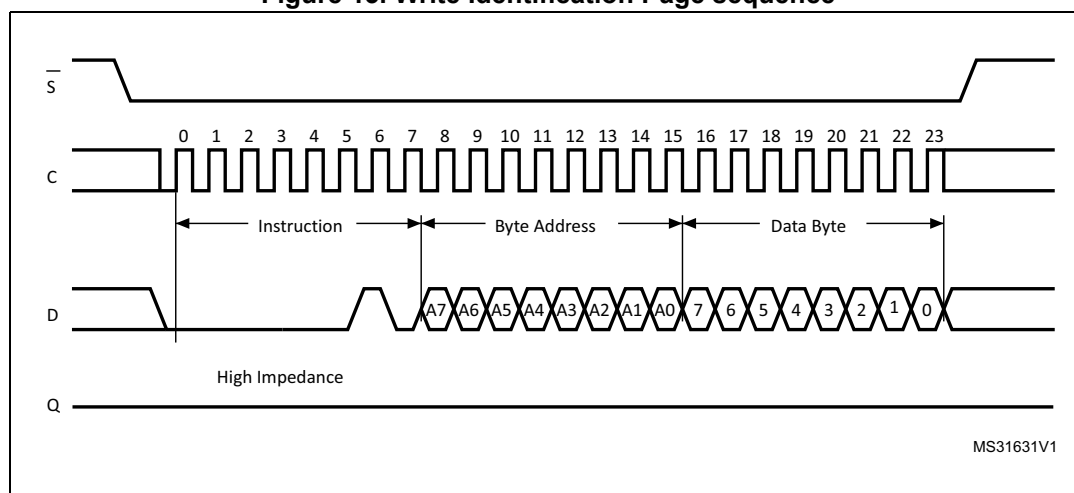
Figure 13. Write Identification Page sequence
