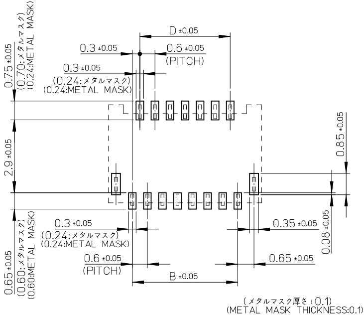
推奨基板寸法 RECOMMENDED P.W.B. PATTERN LAYOUT
