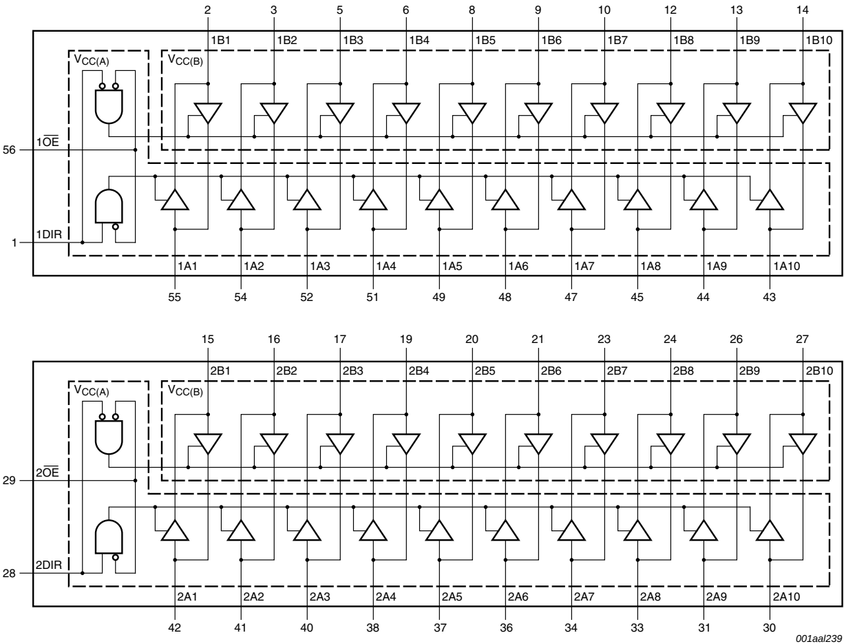
Fig 2. Logic symbol
