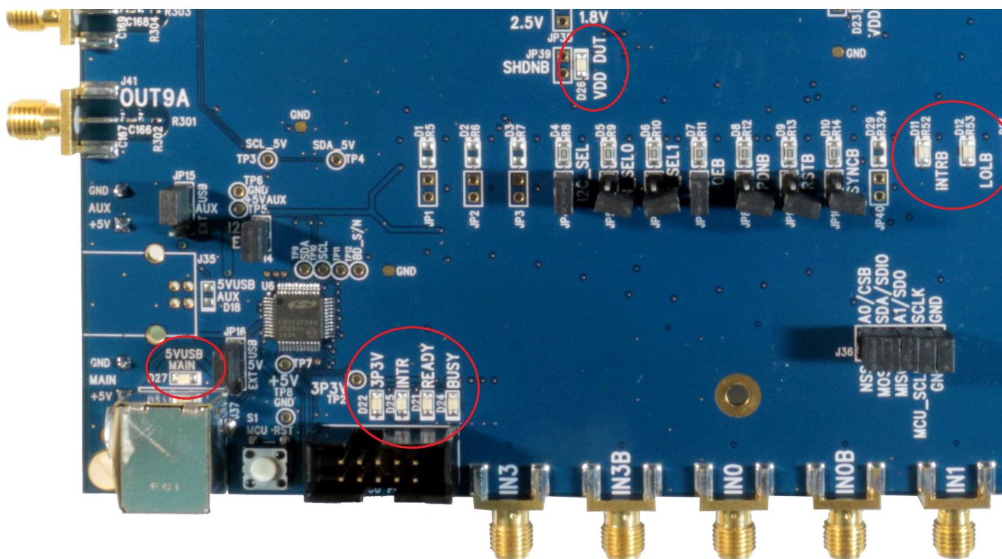
Figure 3.1. Status LEDs
