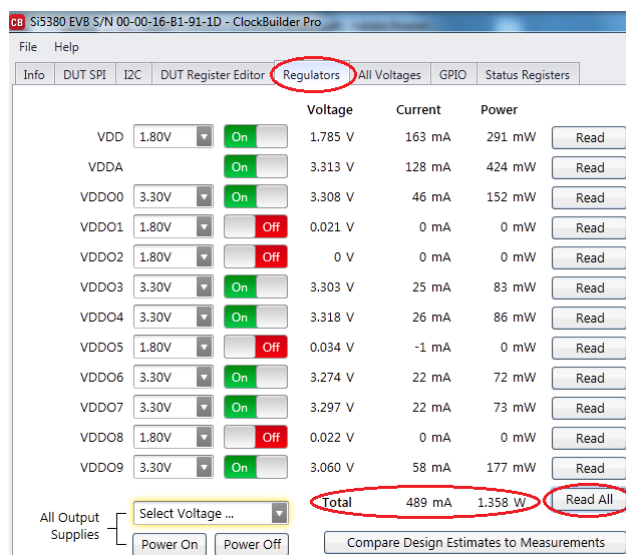
Figure 6.11. EVB GUI—Regulators
