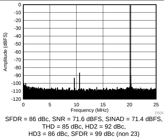
Figure 36. FFT for 170-MHz Input Signal (Dither On)
