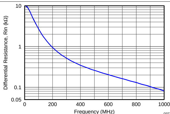
Figure 77. ADC Analog Input Resistance ( R_{IN} ) Across Frequency
