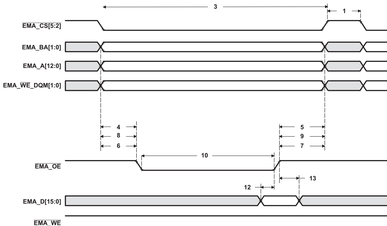
Figure 6-13. Asynchronous Memory Read Timing for EMIFA
