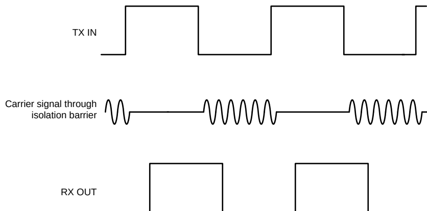
Figure 12. On-Off Keying (OOK) Based Modulation Scheme
