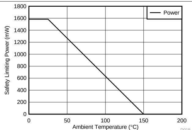
Figure 16. Thermal Derating Curve for Safety Limiting Power per VDE
