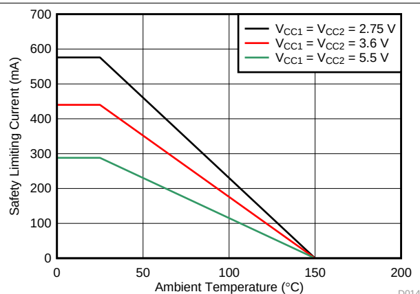
Figure 15. Thermal Derating Curve for Safety Limiting Current per VDE
