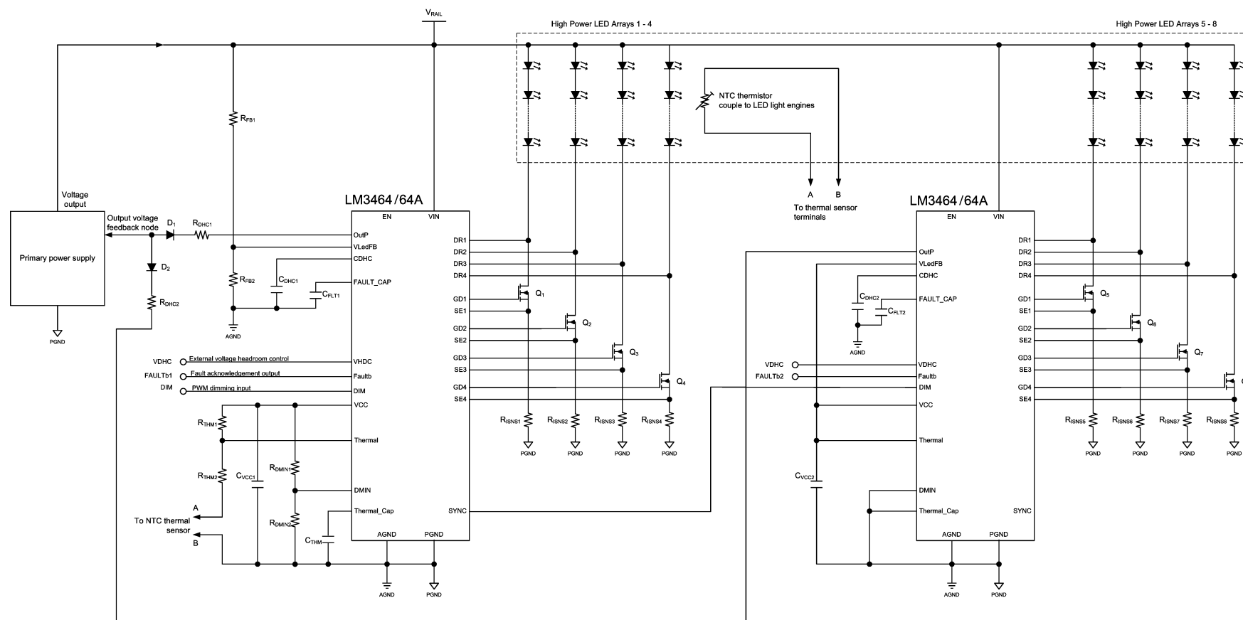
Figure 27. Cascade Operation with Thermal Foldback Control
