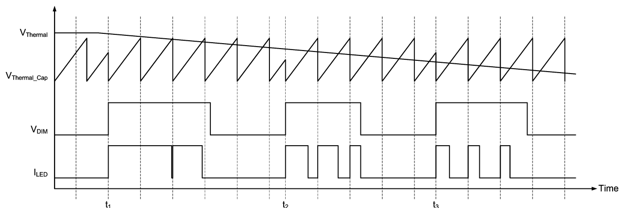
Figure 24. Thermal Foldback + PWM Dimming Control
