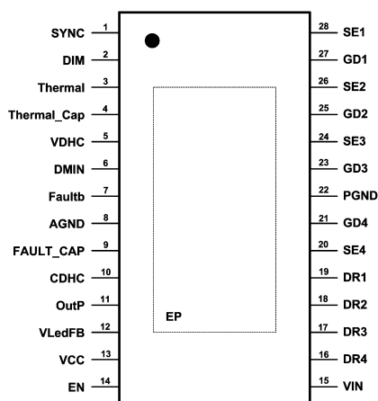
Figure 1. Top View 28-Lead TSSOP-28 Package Number PWP
