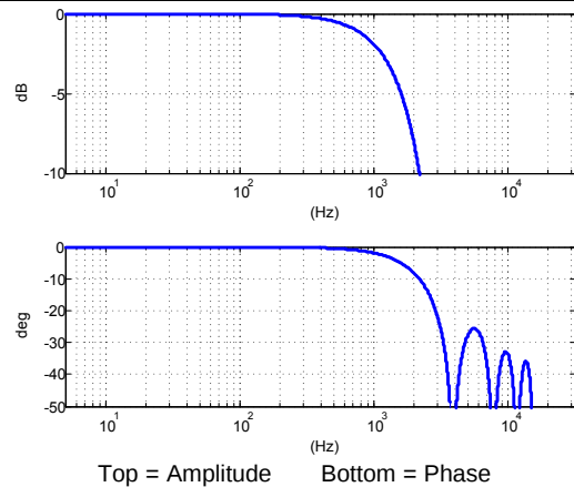
Figure 25. Frequency Response of the 2nd Stage Decimator at Sample Output Rate of 256 \mu s Per Sample
