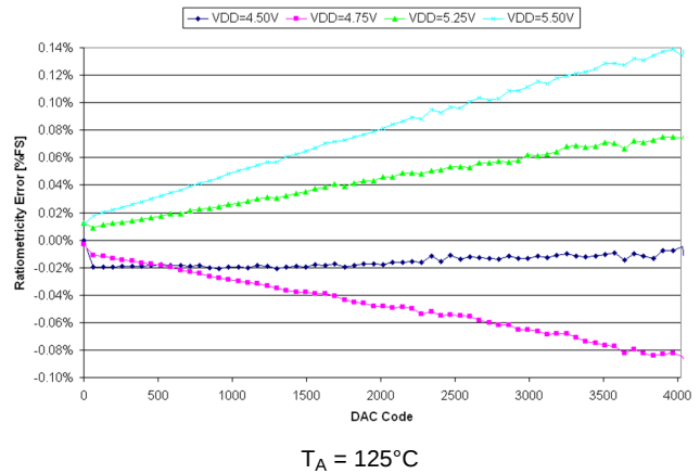
Figure 19. DAC2, Ratiometric Error vs DAC Code
