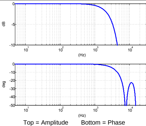
Figure 24. Frequency Response of the 2nd Stage Decimator at Sample Output Rate of 128 \mu s Per Sample
