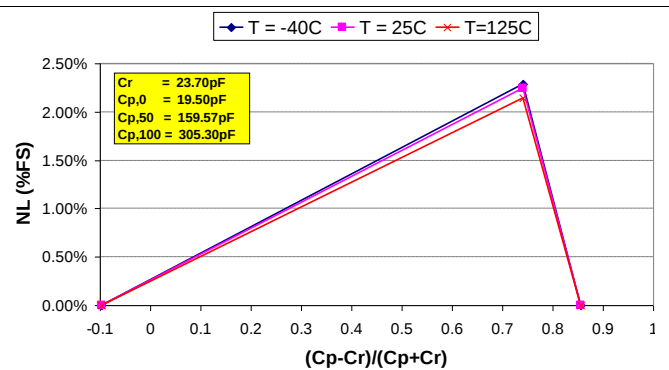
Figure 11. Linearity (%FS)
