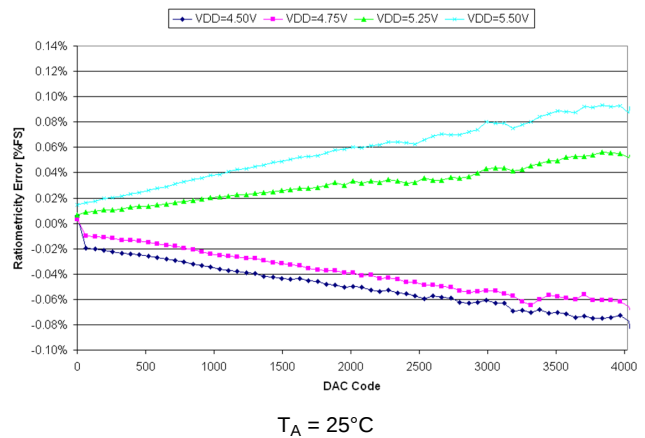
Figure 17. DAC2, Ratiometric Error vs DAC Code
