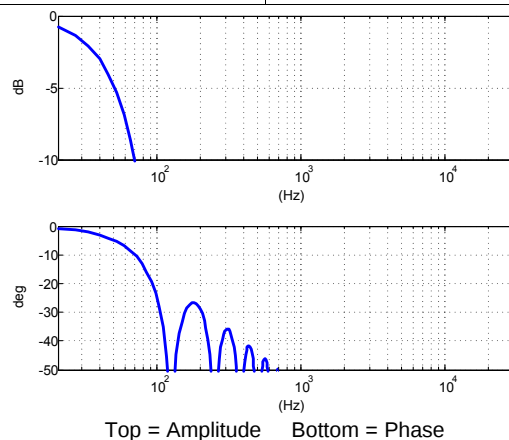
Figure 26. Frequency Response of the Temperature Channel Decimator
