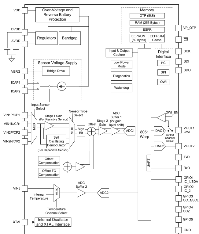
Figure 1. Simplified Schematic
