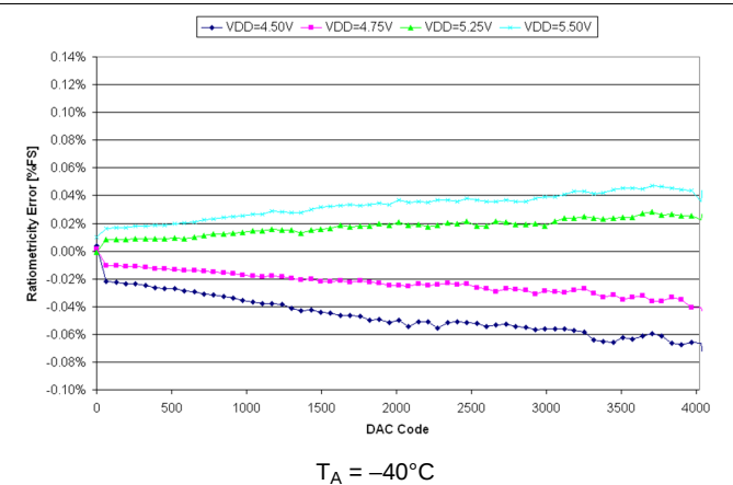
Figure 15. DAC2, Ratiometric Error vs DAC Code
