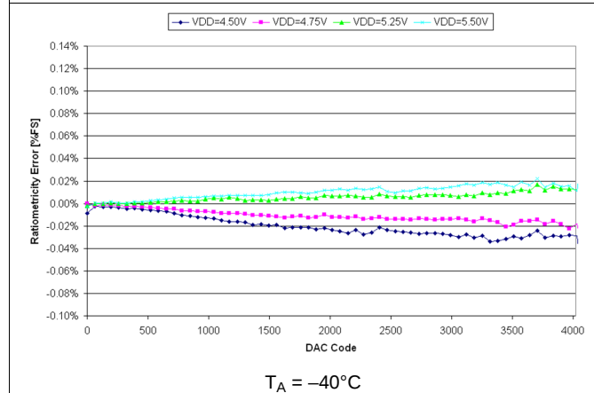
Figure 14. DAC1, Ratiometric Error vs DAC Code
