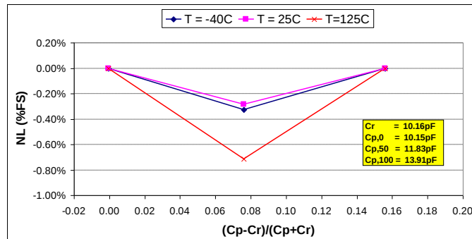
Figure 10. Linearity (%FS)
