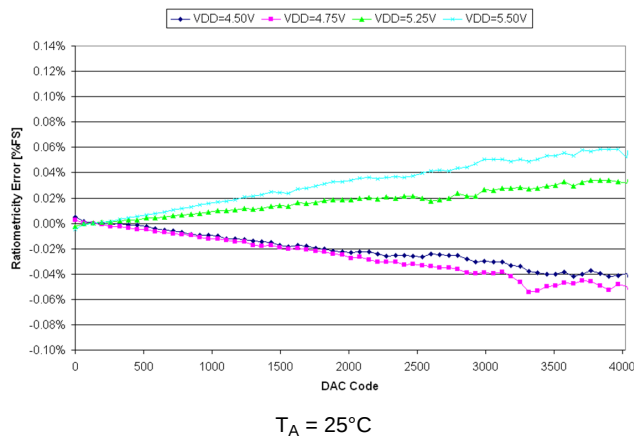
Figure 16. DAC1, Ratiometric Error vs DAC Code
