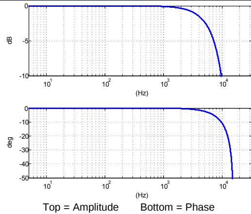
Figure 23. Frequency Response of the 2nd Stage Decimator at Sample Rate of 64 \mu s Per Sample
