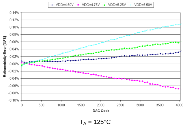
Figure 18. DAC1, Ratiometric Error vs DAC Code
