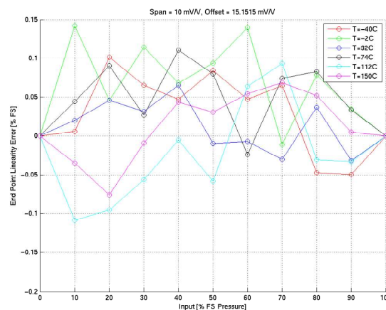
Figure 5. Typical %NL Temperature Drift Characteristics
