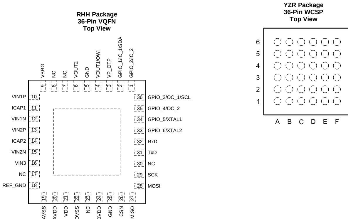
Pin Functions - RHH Package
