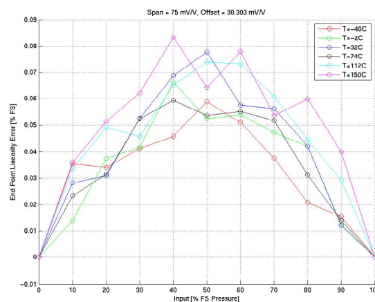
Figure 7. Typical %NL Temperature Drift Characteristics
