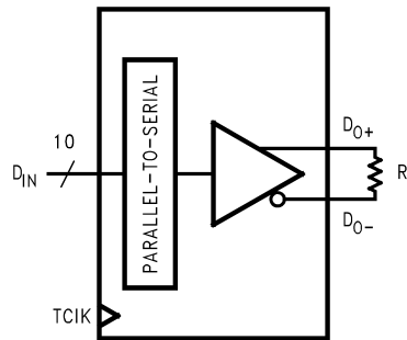
Figure 19. V_{OD} Diagram
