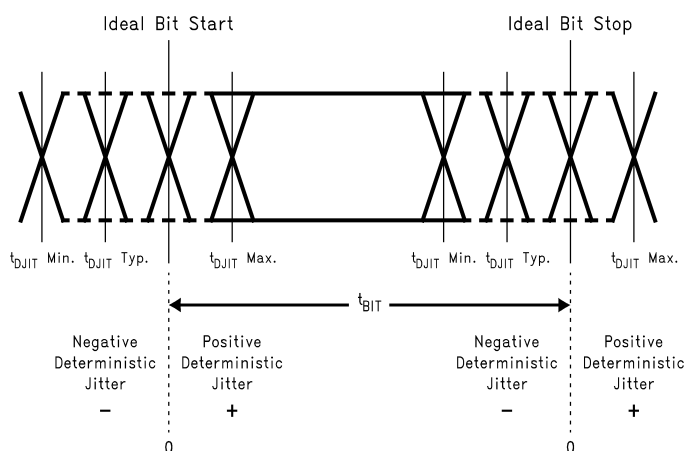
Figure 21. Deterministic Jitter and Ideal Bit Position
