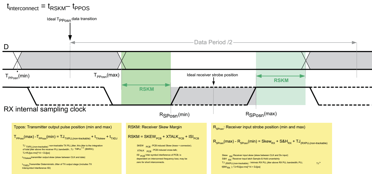
Figure 30. Jitter Budget
