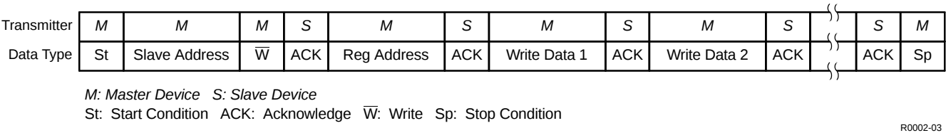
Figure 53. Framework for Write Operation
