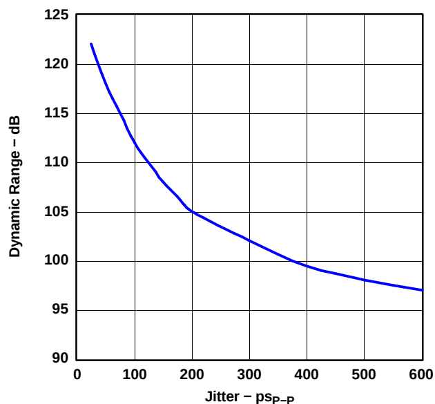
Figure 42. Clock Jitter
