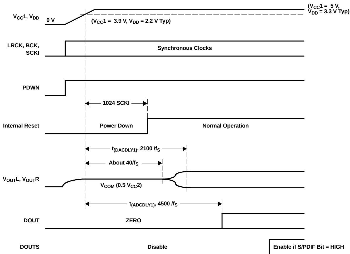
Figure 44. DAC Output and ADC Output for Power-On Reset
