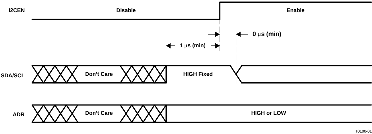
Figure 54. I2CEN Timing Chart
