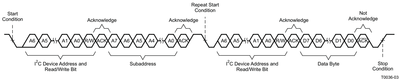
Figure 48. Read Transfer
