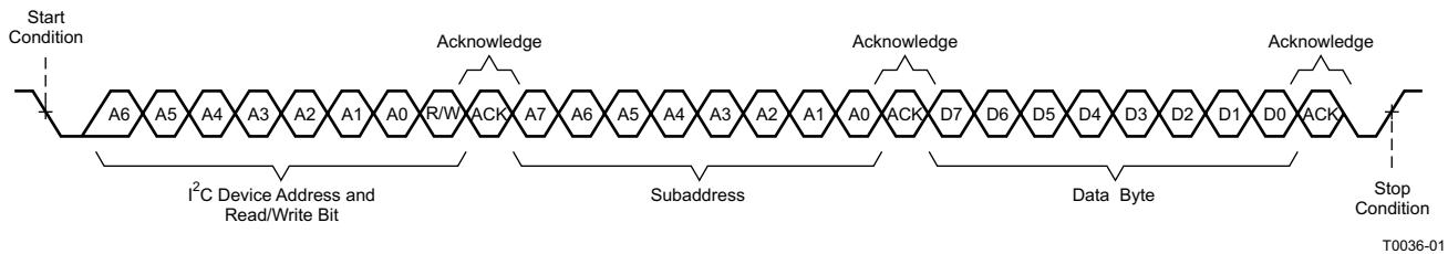
Figure 47. Write Transfer
