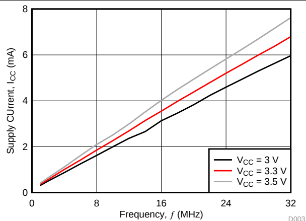
Figure 12. Supply Current vs Frequency ( V_{CC} = 3, 3.3 , and 3.5\text{ V} )
