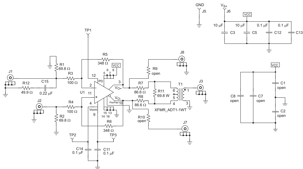
Figure 62. THS4508 EVAL1 EVM Schematic
