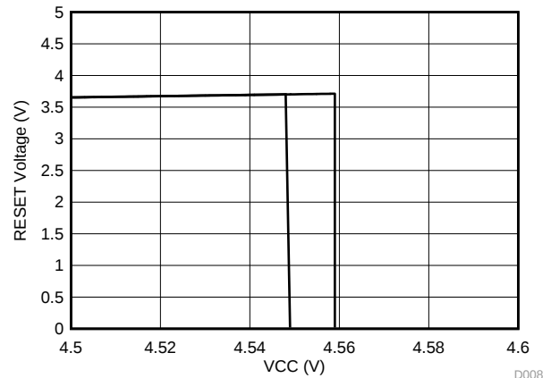
Figure 12. Supervisor RESET Output Voltage vs V_{CC} at Transition
