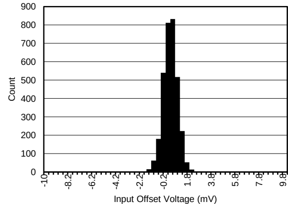
Figure 27. Input Offset Voltage Histogram
