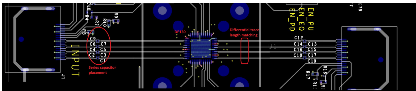
Figure 38. Layout Example
