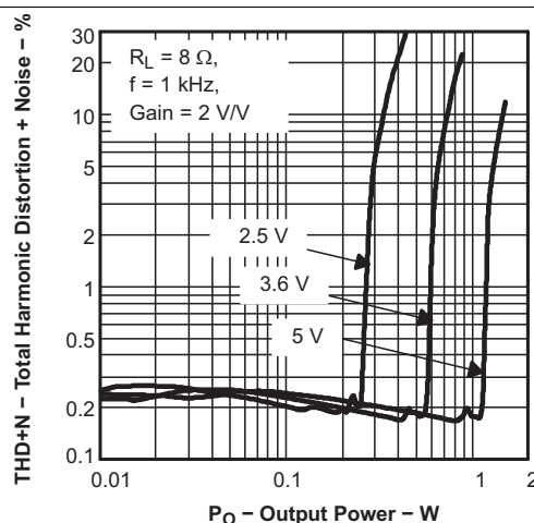
Figure 14. Total Harmonic Distortion + Noise vs Output Power
