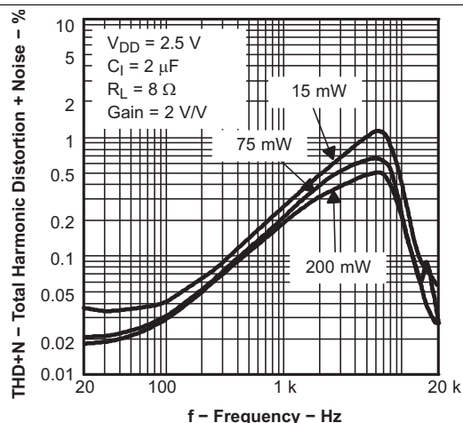
Figure 18. Total Harmonic Distortion + Noise vs Frequency
