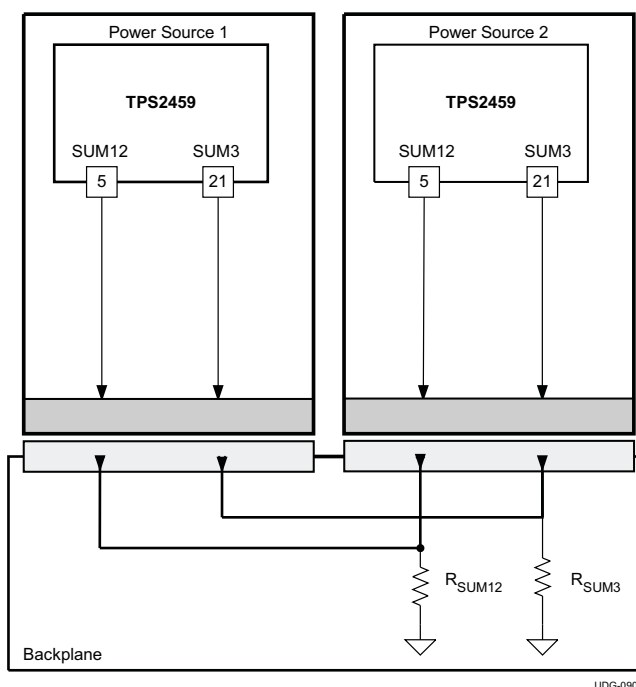
Figure 27. Multiswap Redundancy
