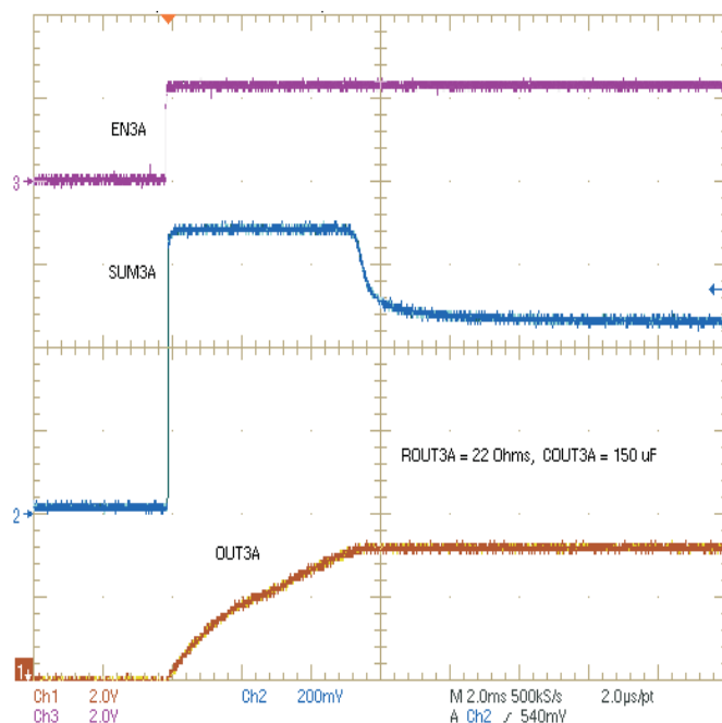
Figure 10. OUT3 Startup Into 22- \Omega , (150 mA), 150- \mu F Load
