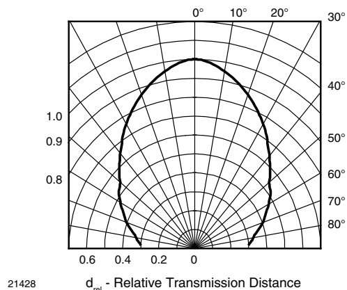
Fig. 4 - Vertical Directivity
