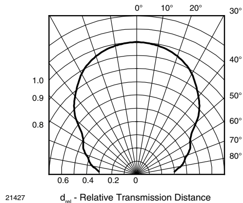
Fig. 3 - Horizontal Directivity
