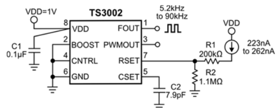
Figure 2: Configuring the TS3002 into a Current-Controlled Oscillator.
