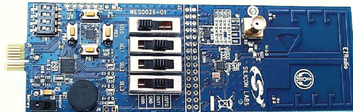
Figure 5. EZRadio RFStick Receiver Board (P/N 4356-LED-434-DIR)
