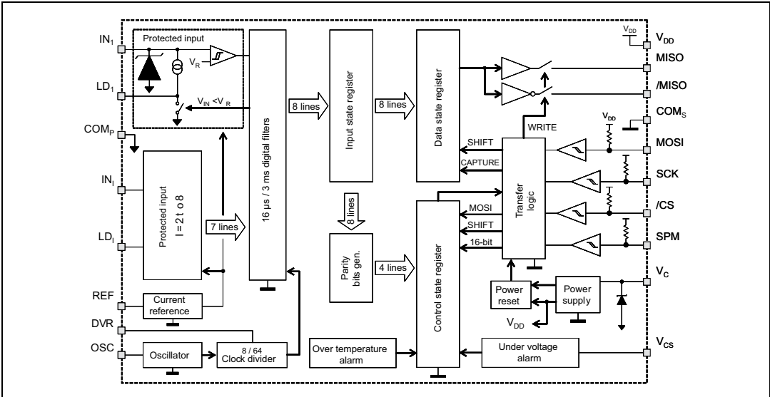
Figure 1. circuit block diagram
