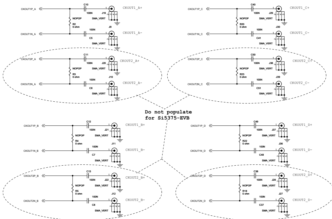
Figure 6. Clock Outputs
