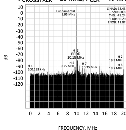
Crosstalk Response f_{IN} = 9.95\text{ MHz} , f_{CROSSTALK} = 15\text{ MHz} , f_{CLK} = 40\text{ MHz}
