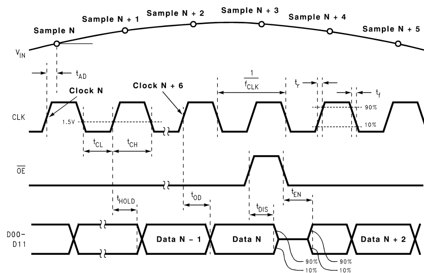
Figure 3. Output Timing
