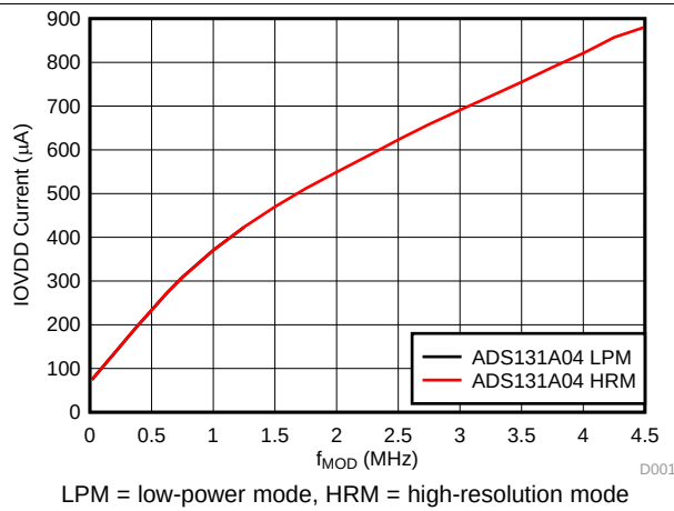
Figure 28. ADS131A04 IOVDD Current vs f_{MOD}
