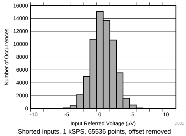
Figure 5. Single Device Noise Histogram
