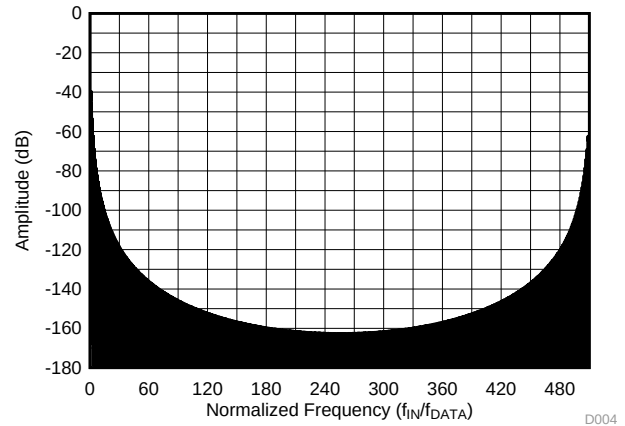
Figure 42. Sinc 3 Filter Frequency Response (OSR 512)
