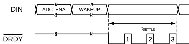
Figure 45. \text{sinc}^3 Filter Settling
