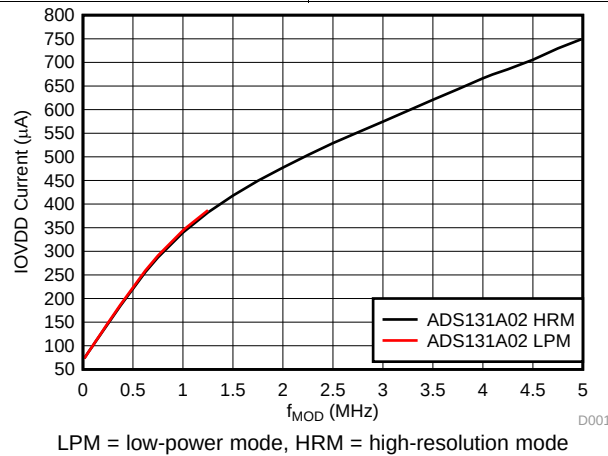
Figure 30. ADS131A02 IOVDD Current vs f_{MOD}
