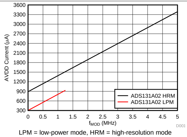
Figure 29. ADS131A02 AVDD Current vs f_{MOD}
