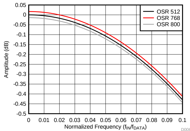
Figure 44. Non-Binary OSR \text{sinc}^3 Filter Frequency Response
