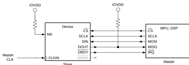
Figure 57. Asynchronous Interrupt Mode Device Connections
