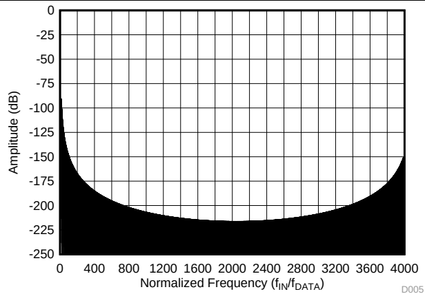
Figure 43. Sinc 3 Filter Frequency Response (OSR 4096)
