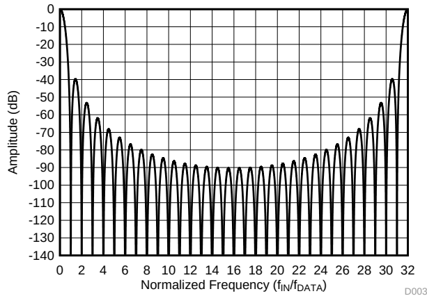
Figure 41. Sinc 3 Filter Frequency Response (OSR 32)
