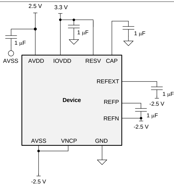
Figure 110. Bipolar Analog Power Supply
