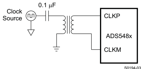
Figure 41. Differential Clock
